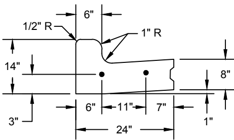
SECTION A1-A1
