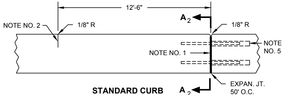
8" CURB & GUTTER PLAN VIEW
