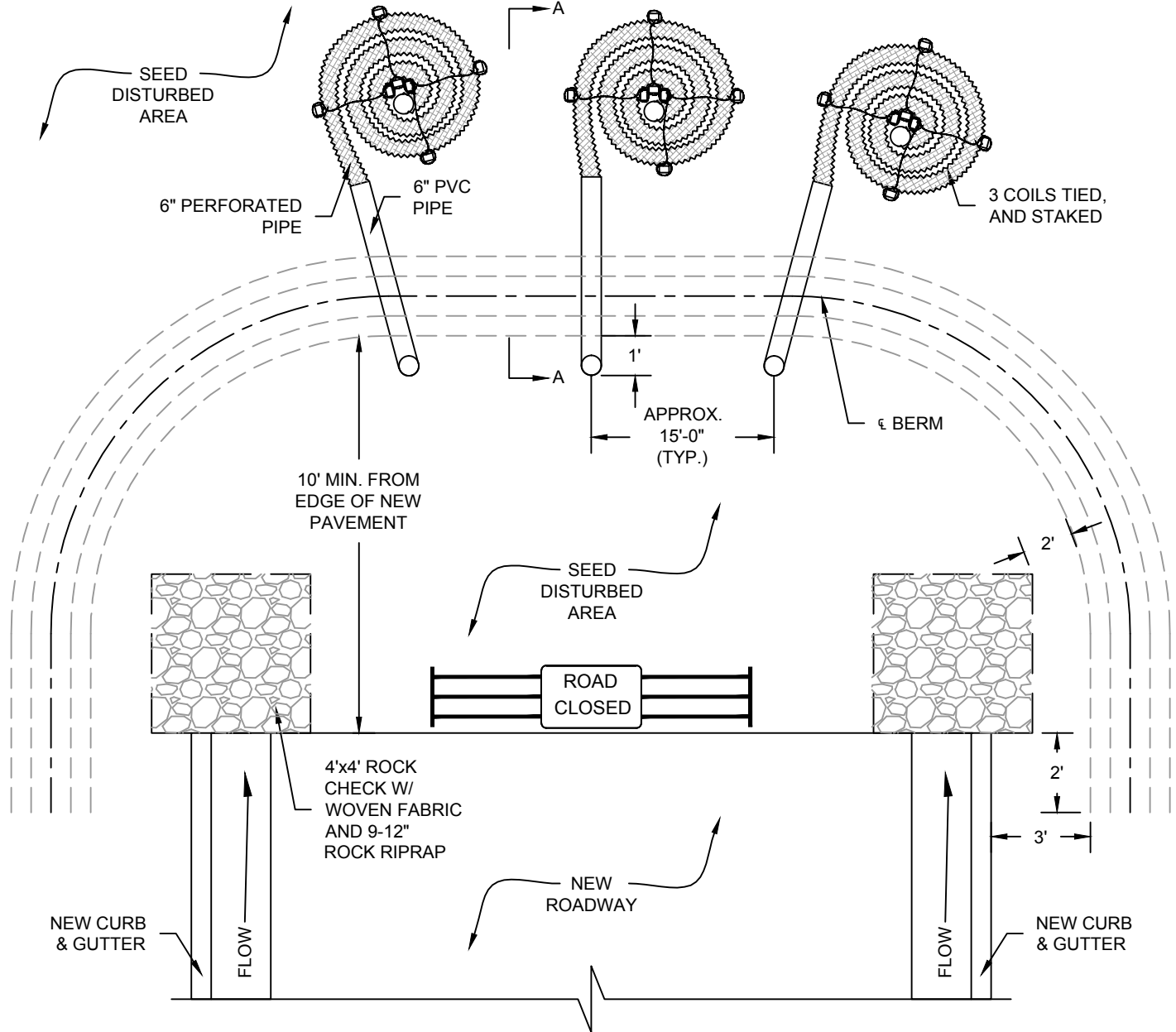
PLAN VIEW
